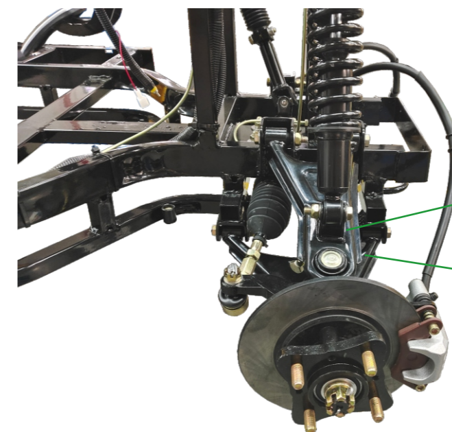
2 NEW STAMPING A-ARM, LOWER 3 NEW STAMPING A-ARM, LOWER
